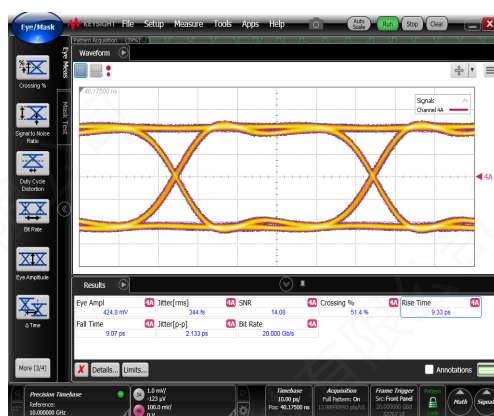
Input signal Eye amplitude = 0.43 \text{ V}_{\text{pp}}
