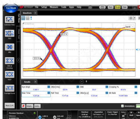
Output response Eye amplitude = 6 \text{ V}_{\text{pp}}
